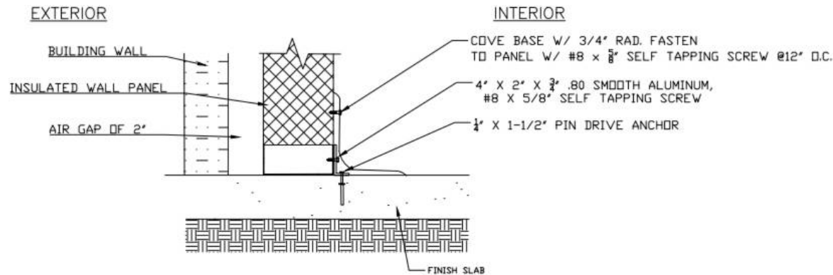
WALL TO FLOOR CONNECTION
