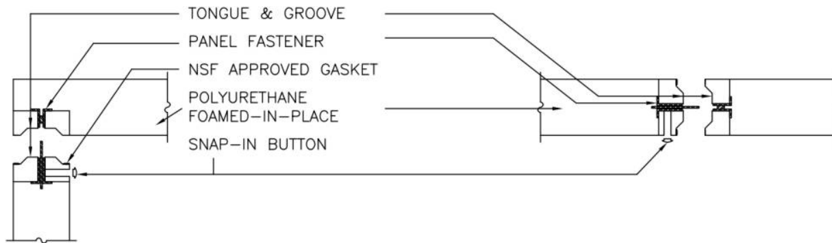
DETAIL #3
