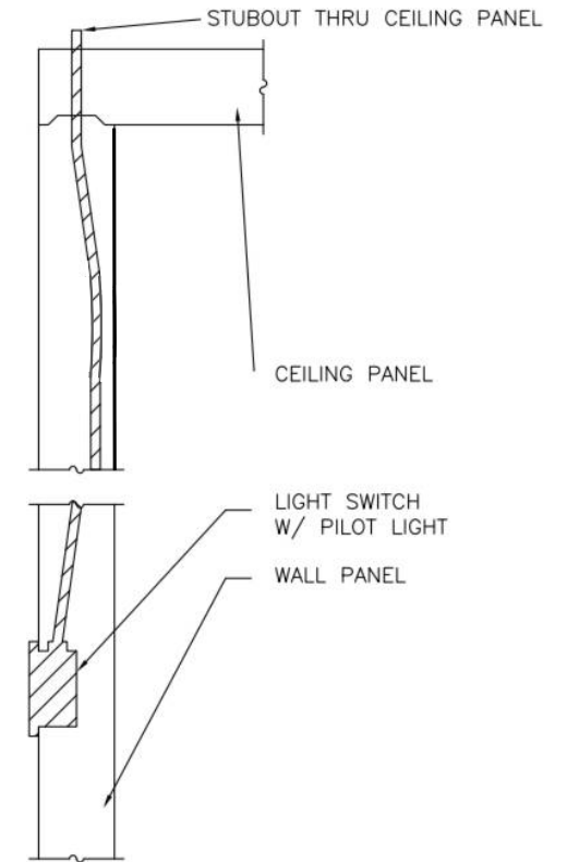
LIGHT SWITCH TO LIGHT FIXTURE CONNECTION (LOOSE)
